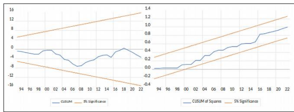
Figure 1: CUSUM and CUSUMSQ test for stability diagnostic.
