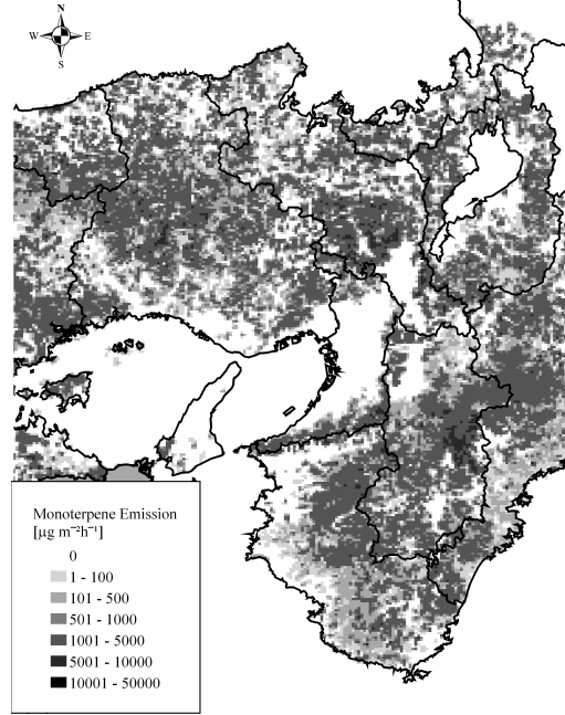
Figure 1b: Standard emissions of monoterpene in Kinki region
