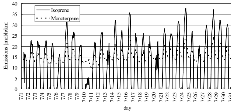
Figure 2: Hourly variations of isoprene and monoterpene
