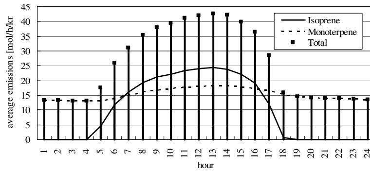
Figure 3: hourly average emissions
