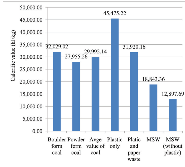
Fig. 5: Calorific values of different samples
