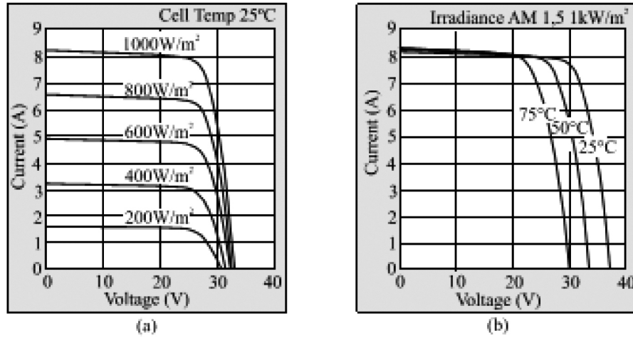
Fig. 1: I-V curve from Kyocera KC200GT PV module: (a) under constant temperature and (b) under constant irradiance
