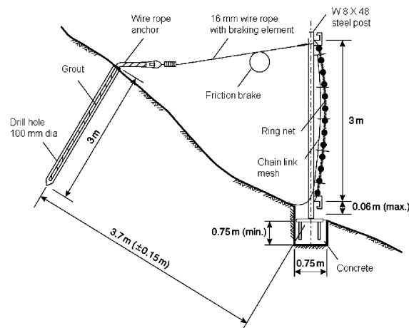
Fig. 6. Schematic of Rockfall barrier system discussed herein. Modified after [26] and courtesy Geobrugg Inc.
